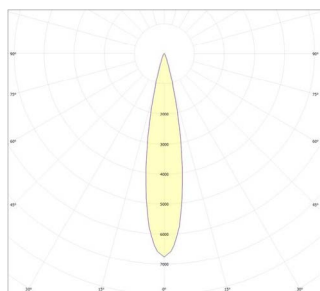
20° Beam Distribution
