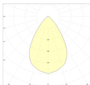
67° Beam Distribution
